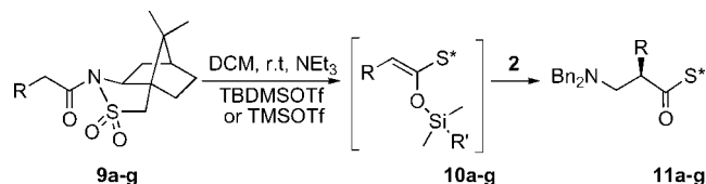
Scheme 6. Aminomethylation of chiral silyl ketene N,O-acetal with the iminium trifluoroacetate salt. S^* = (+)-camphorsultam.
