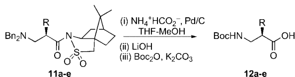
Scheme 7. Deprotection and Boc protection.
