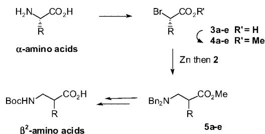
Scheme 2. Synthesis of racemic \beta^2 -amino acids through Reformatsky reactions with the iminium trifluoroacetate salt.
