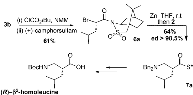
Scheme 3. Synthesis of optically pure \beta^2 -homoleucine through a Reformatsky reaction using the iminium trifluoroacetate salt. S* = (+)-camphorsultam.
