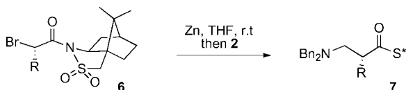
Scheme 5. Asymmetric synthesis of \beta -amino acids through Reformatsky reactions using the iminium trifluoroacetate salt. S^* = (+)-camphorsultam.
